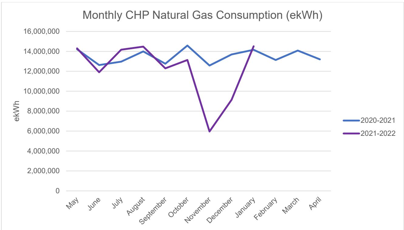
Figure 8: McMaster Monthly Cogeneration (CHP) Natural Gas Consumption (ekWh)
