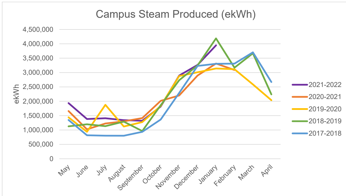
Figure 6: McMaster Campus Steam Production Profile
