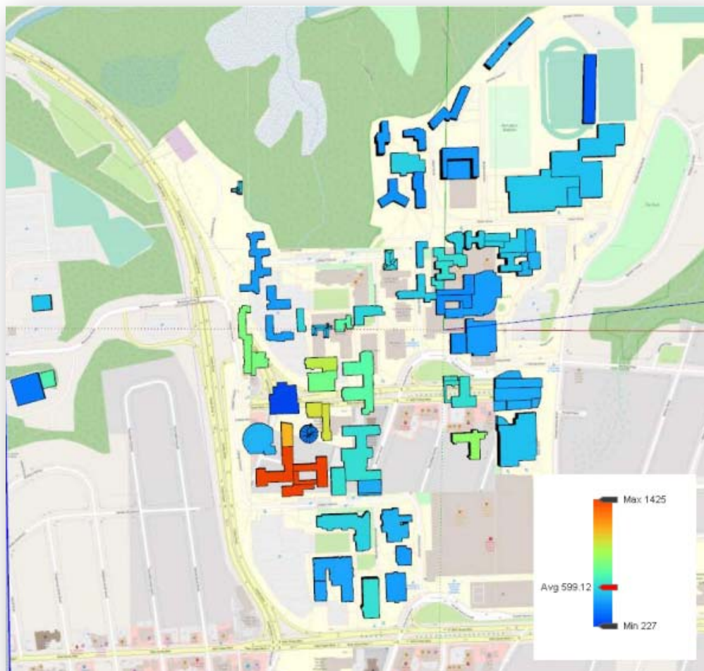
Figure 14: Campus Energy Model [Source: McMaster Net-Zero Carbon Roadmap Report]
